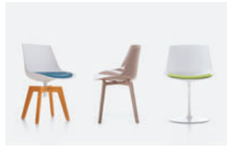
Flow Chair
