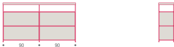
composition 4 L184 D39 H101 cm
