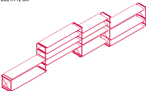
composition S-5 L458 D33 H112 cm
