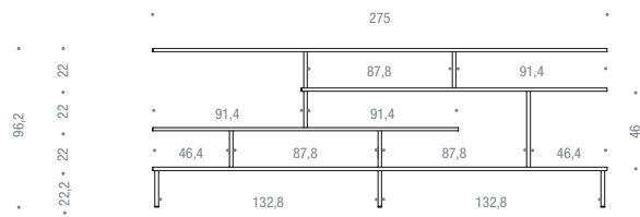
COMPOSITION C | L275 D40 H96.2
