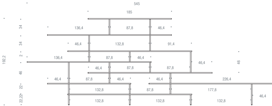
COMPOSITION A | L545 D40 H192.2
