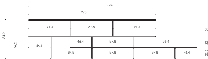
COMPOSITION G | L365 D40 H84.2
