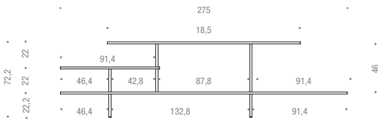
COMPOSITION E | L275 D40 H72.2
