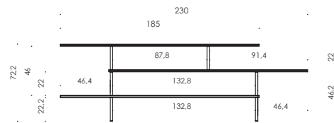
COMPOSITION F | L230 D40 H72.2
