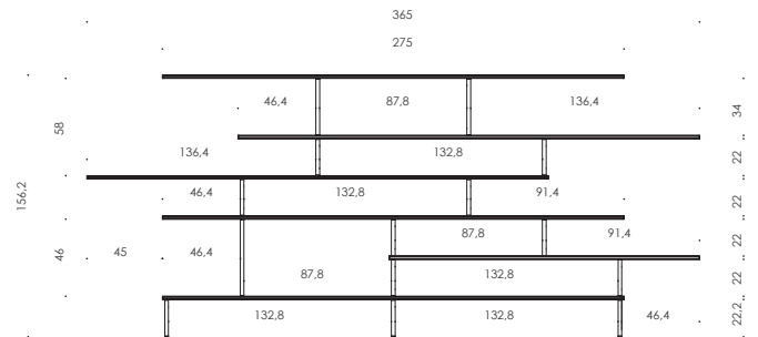
COMPOSITION H | L365 D40 H156.2
